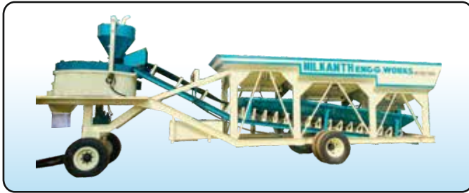
Mobile/Compact Concrete Batching Plant - 3 BIN Cap. 20,30,45,60 Cu.M/Hr.
